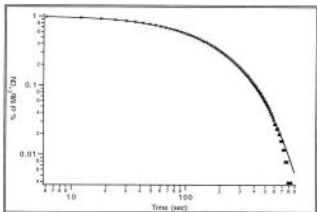
FIGURE 5: Kinetics of dissociation of \text{Fe}^{\text{II}}\text{Mb}-\text{CN} as a function of time at -5^\circ\text{C} . Absorption at 571 nm. Sample conditions given in Figure 4.
